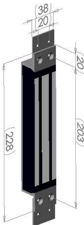
MAGNET BODY DIMENSION
