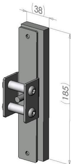
STRIKE PLATE DIMENSION
